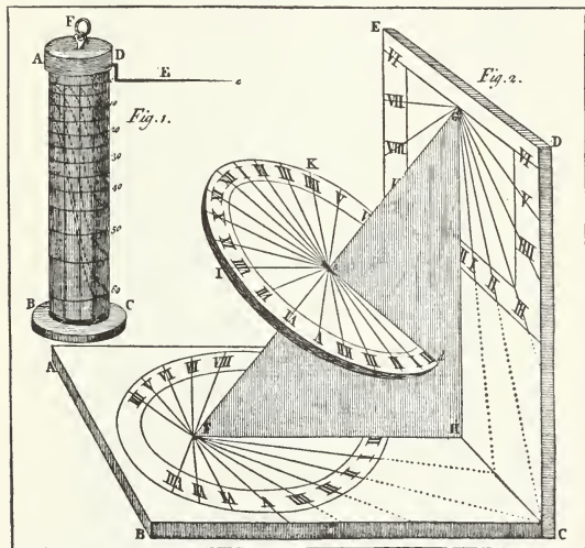
Diagram of Construction of Cylinder-dial.
