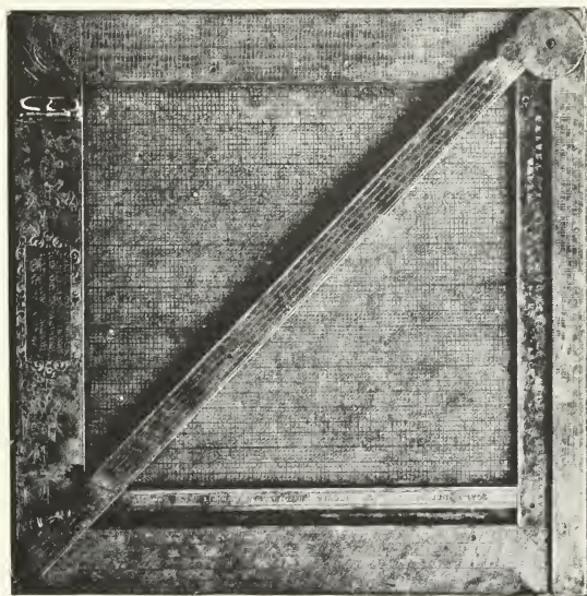
Schissler's Quadrant; Bodleian Library.
